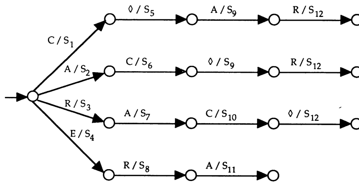
Figure 1. Subgraph of unminimized GADDAG for 'CARE' (see Table I for letter sets)
